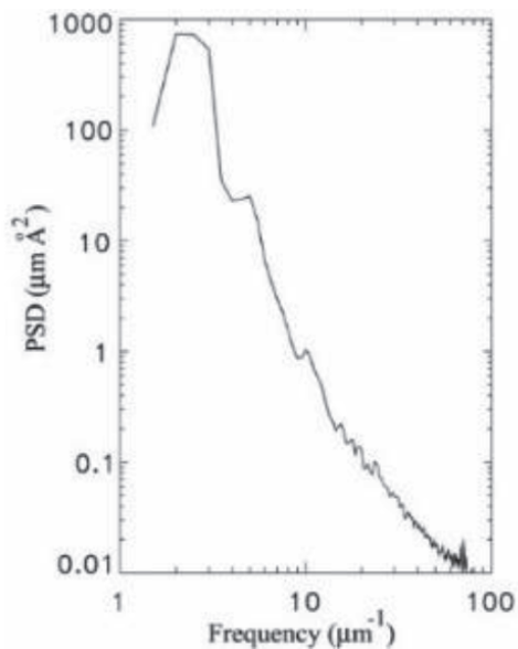
Figure 14. PSD function of 2400/mm replica grating from AFM image (after [31]).
