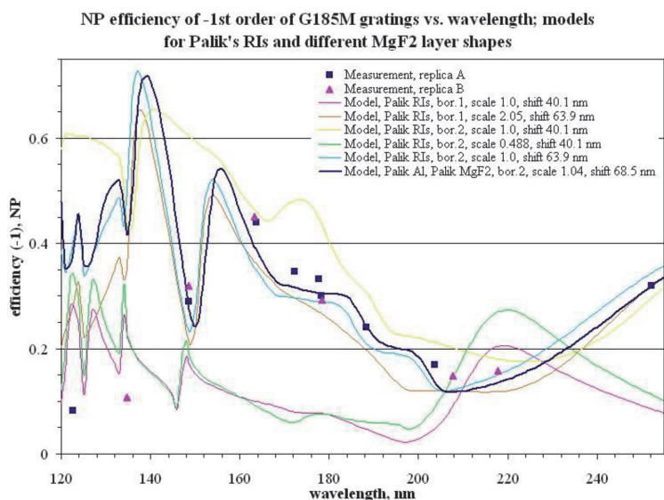
Figure 17. G185M -1st-order NP efficiency measured and calculated for different layer shapes.
