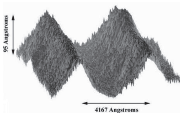
Figure 13. AFM image of 2400/mm replica grating (after [31]).
